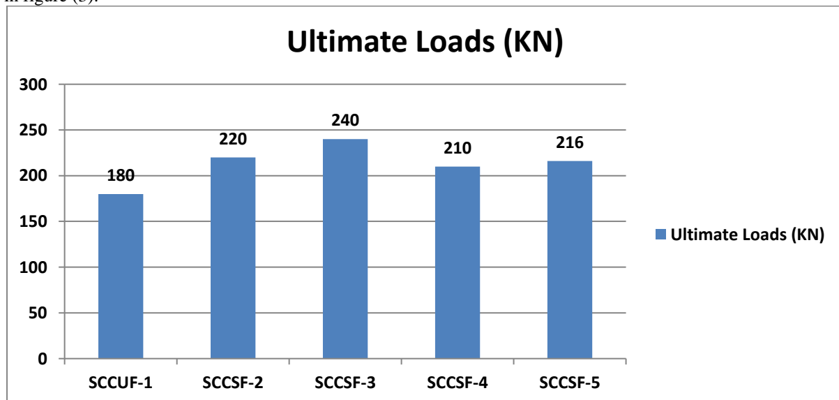
Figure (3): Ultimate loads
